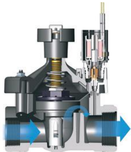
PESB Cutaway
